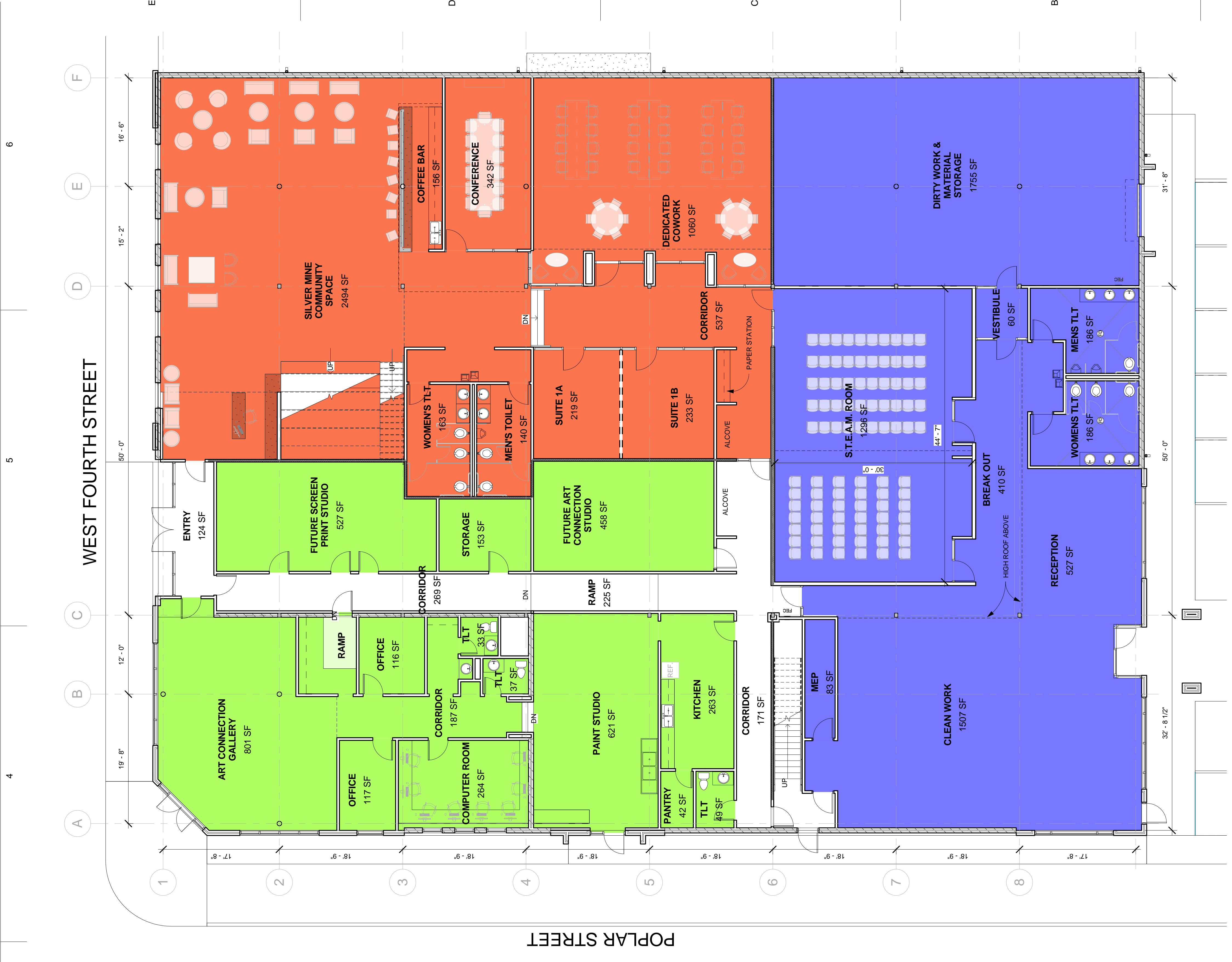
1 PRESENTATION LOWER FLOOR PLAN 1/8" = 1'-0"
