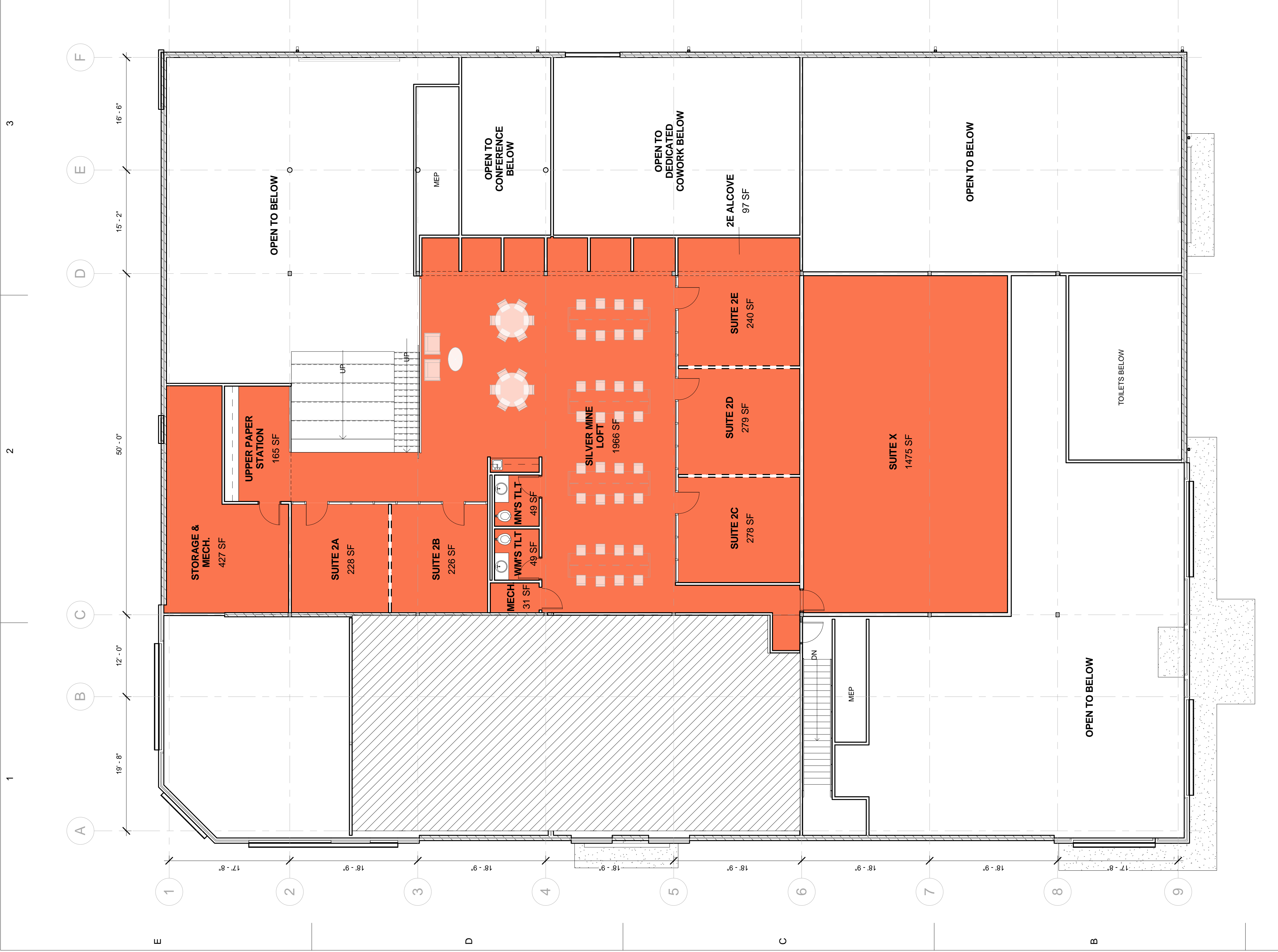
2 PRESENTATION UPPER FLOOR PLAN 1/8" = 1'-0"
